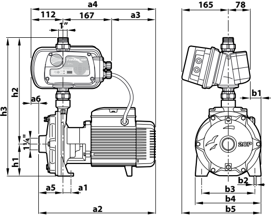
TS1-2CP 25/14 – TS1-2CP 25/16
